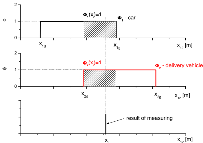
Fig. 2. An example illustrating the formulation of vehicle category models for rectangular (classic) membership functions and the procedure in the event a new result of measuring x_1 is obtained.
