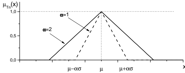
Fig. 3. Interpretation of the triangular MF parameters.
